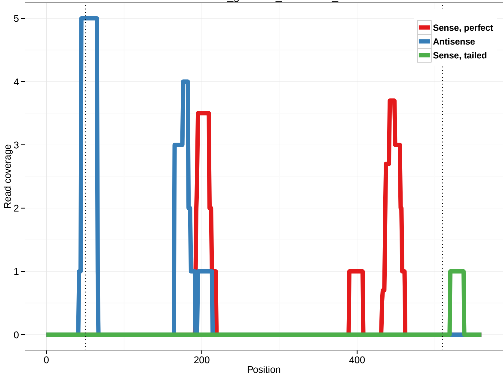
rheMac3_genscan_chr11.542_5
