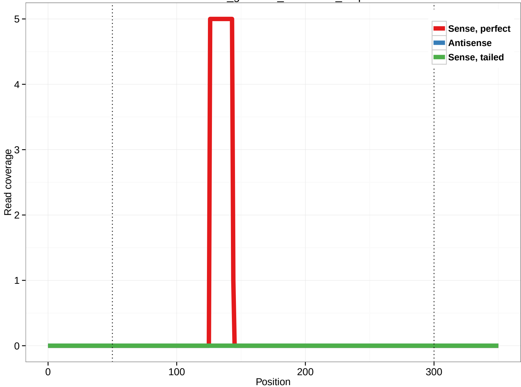
rheMac3_genscan_chr11.513_0.3p
