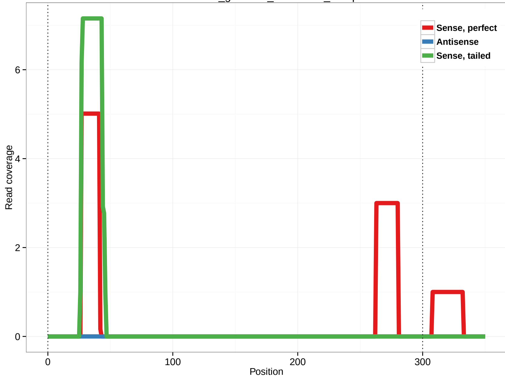
rheMac3_genscan_chr11.428_16.3p
