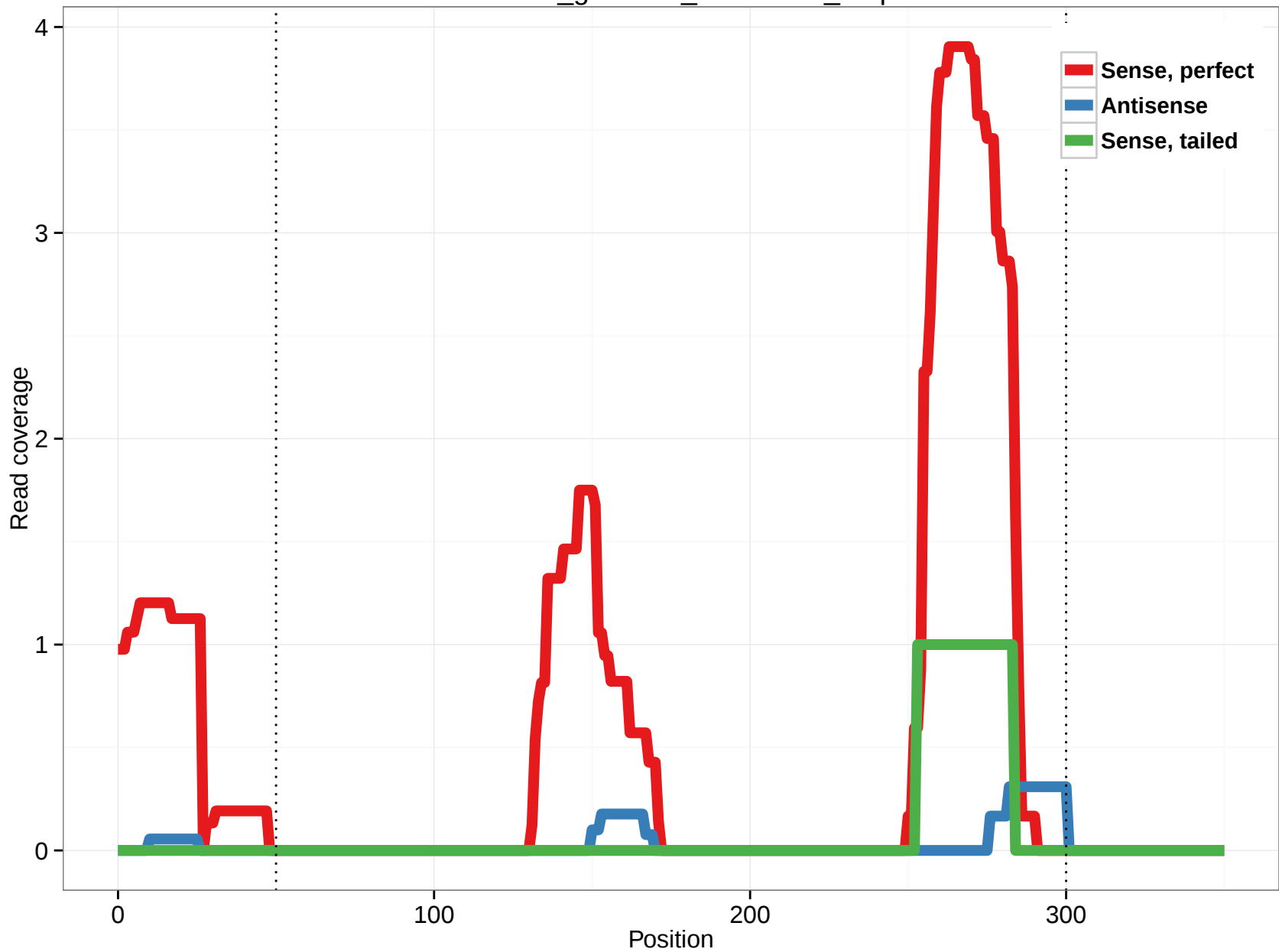
rheMac3_genscan_chr11.407_3.5p
