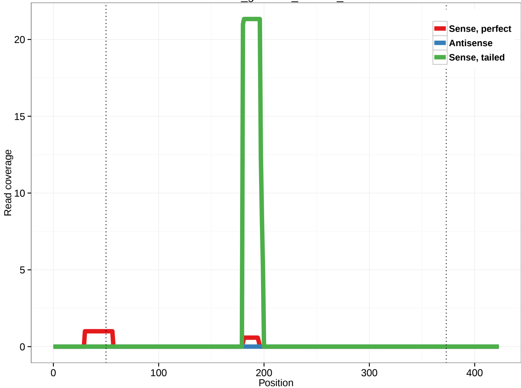
rheMac3_genscan_chr11.3_21
