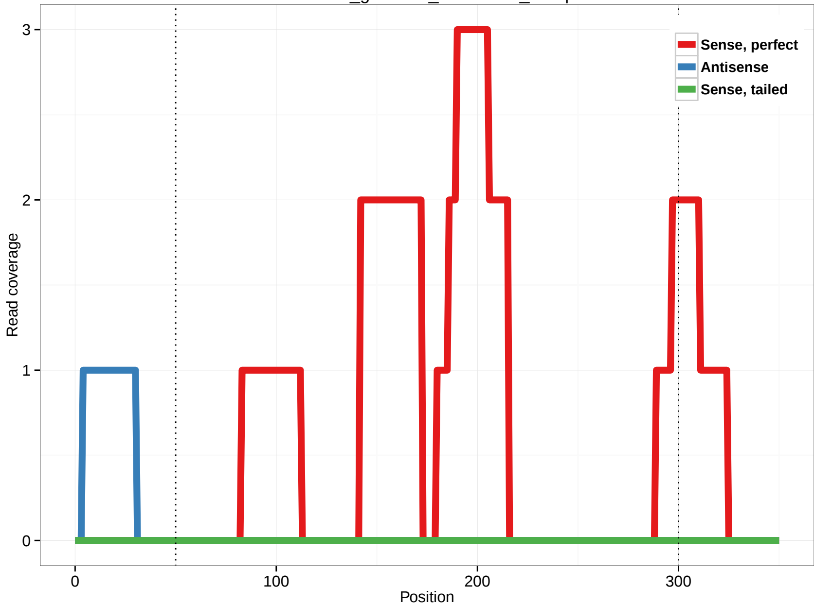
rheMac3_genscan_chr11.337_10.3p
