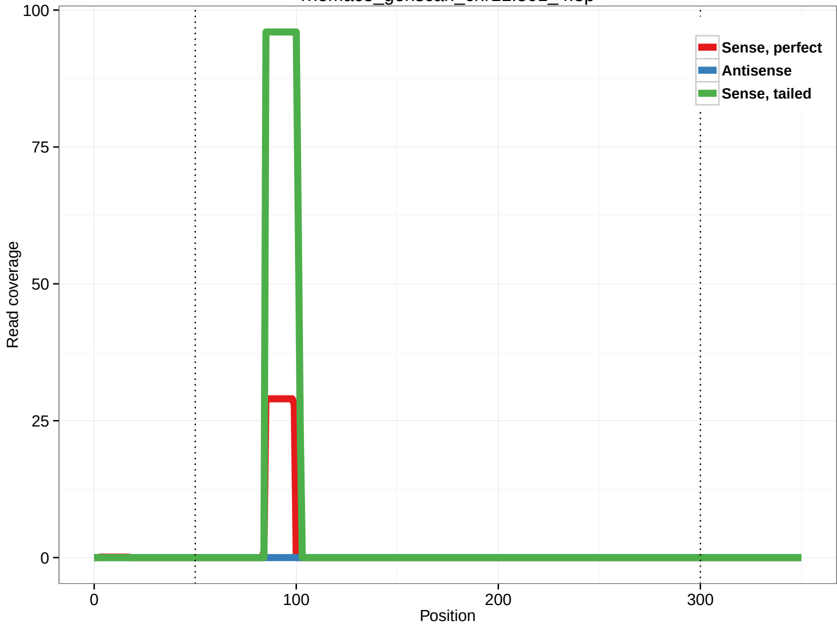
rheMac3_genscan_chr11.301_4.3p
