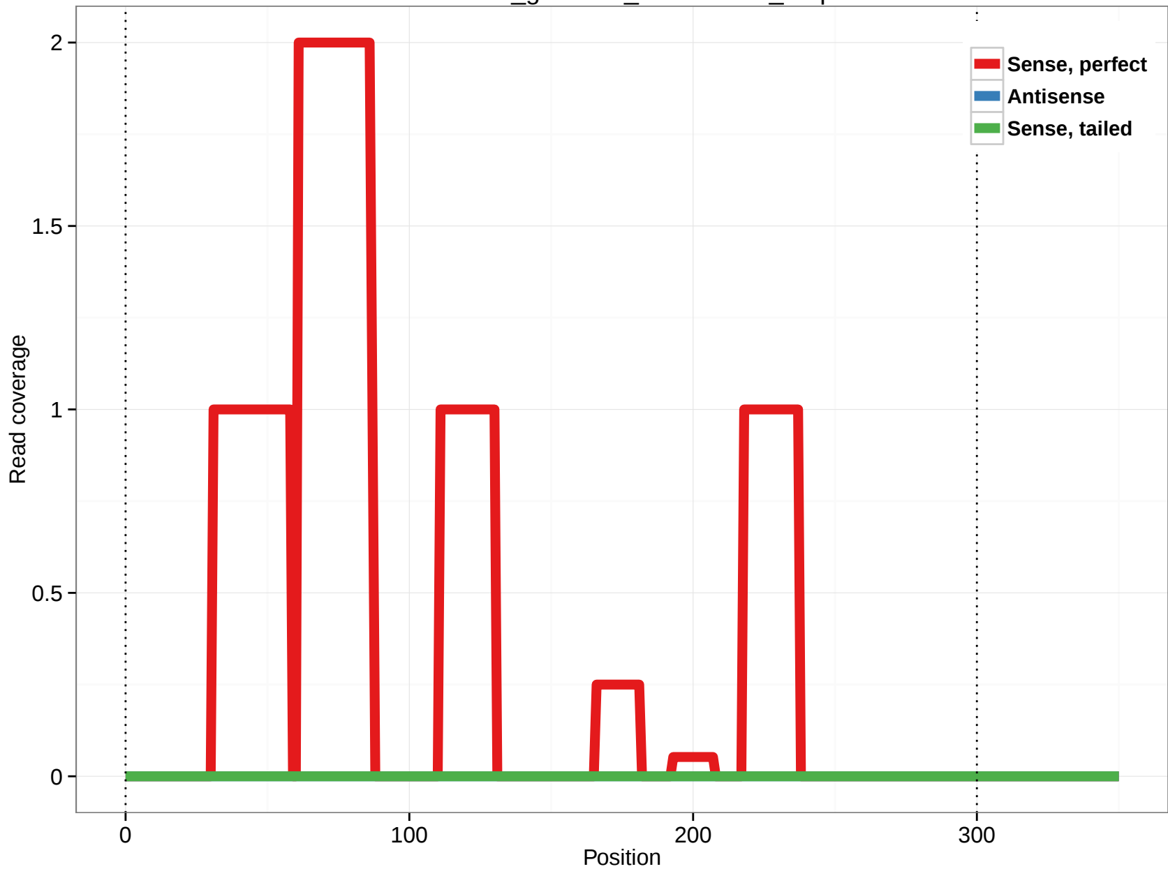
rheMac3_genscan_chr11.2534_3.3p
