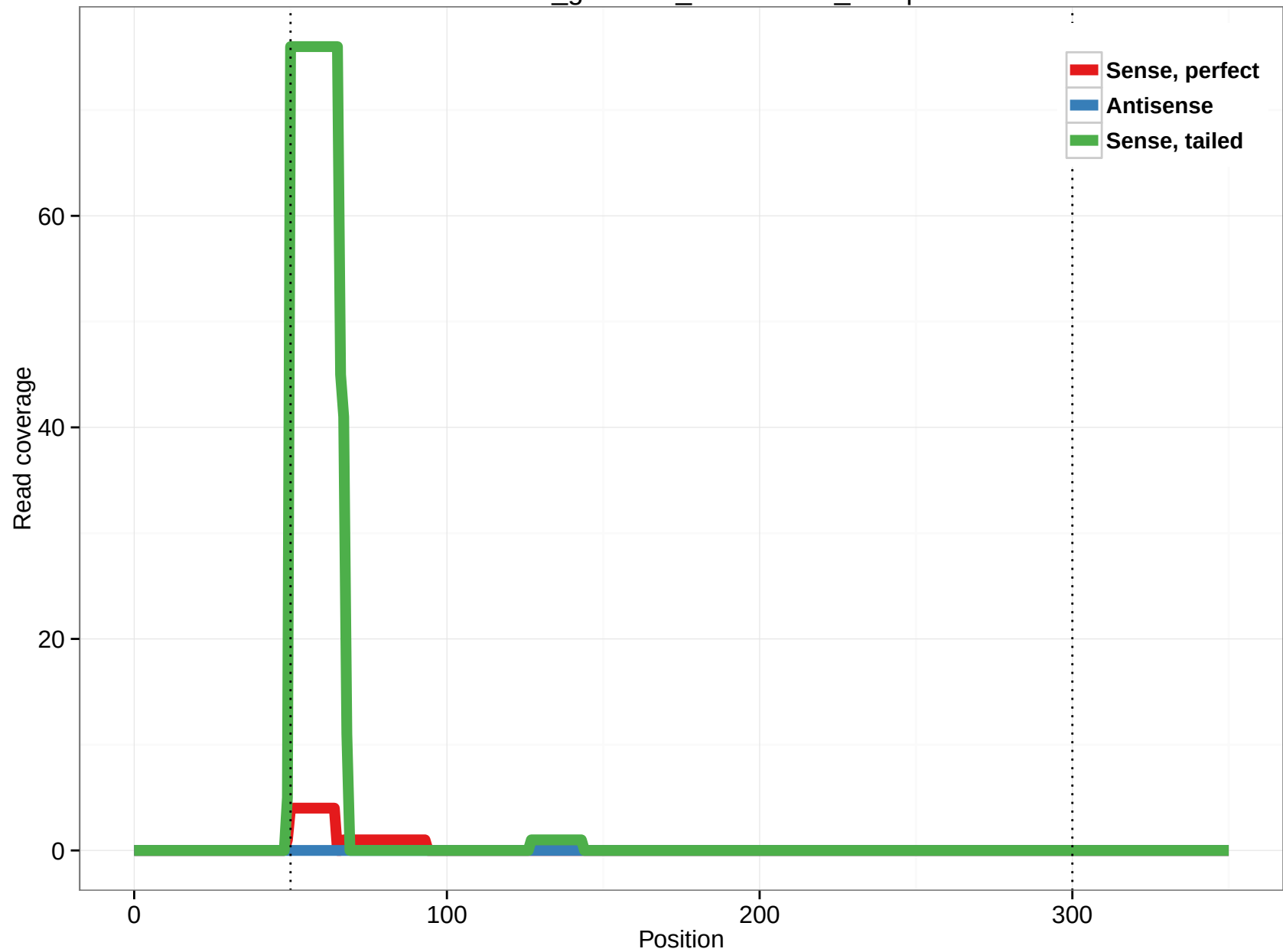
rheMac3_genscan_chr11.2517_30.5p
