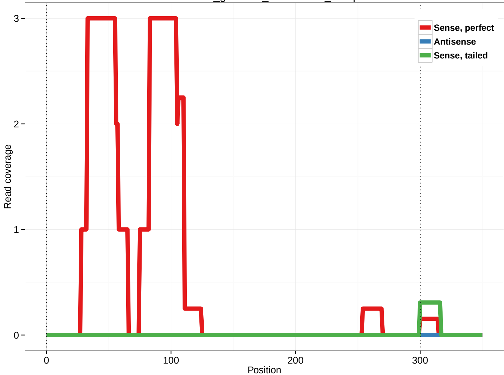
rheMac3_genscan_chr11.2501_54.3p
