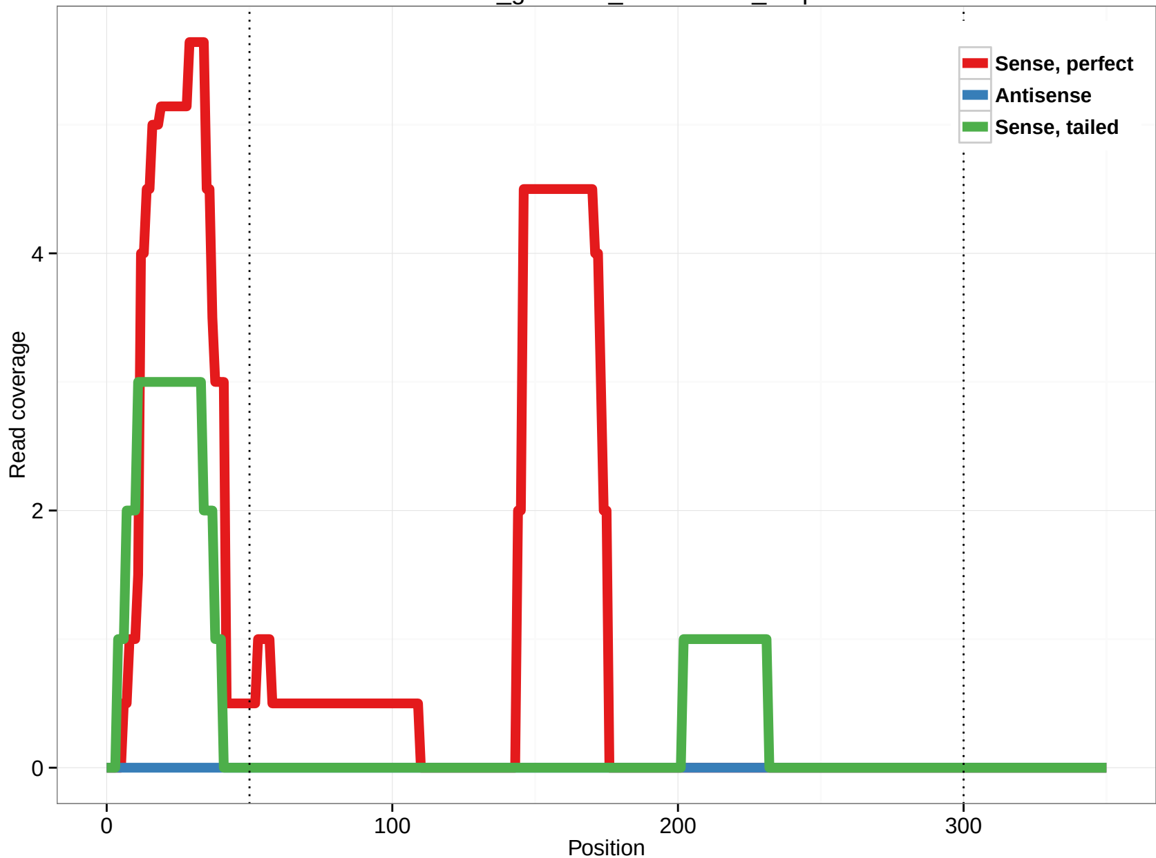
rheMac3_genscan_chr11.2501_0.5p
