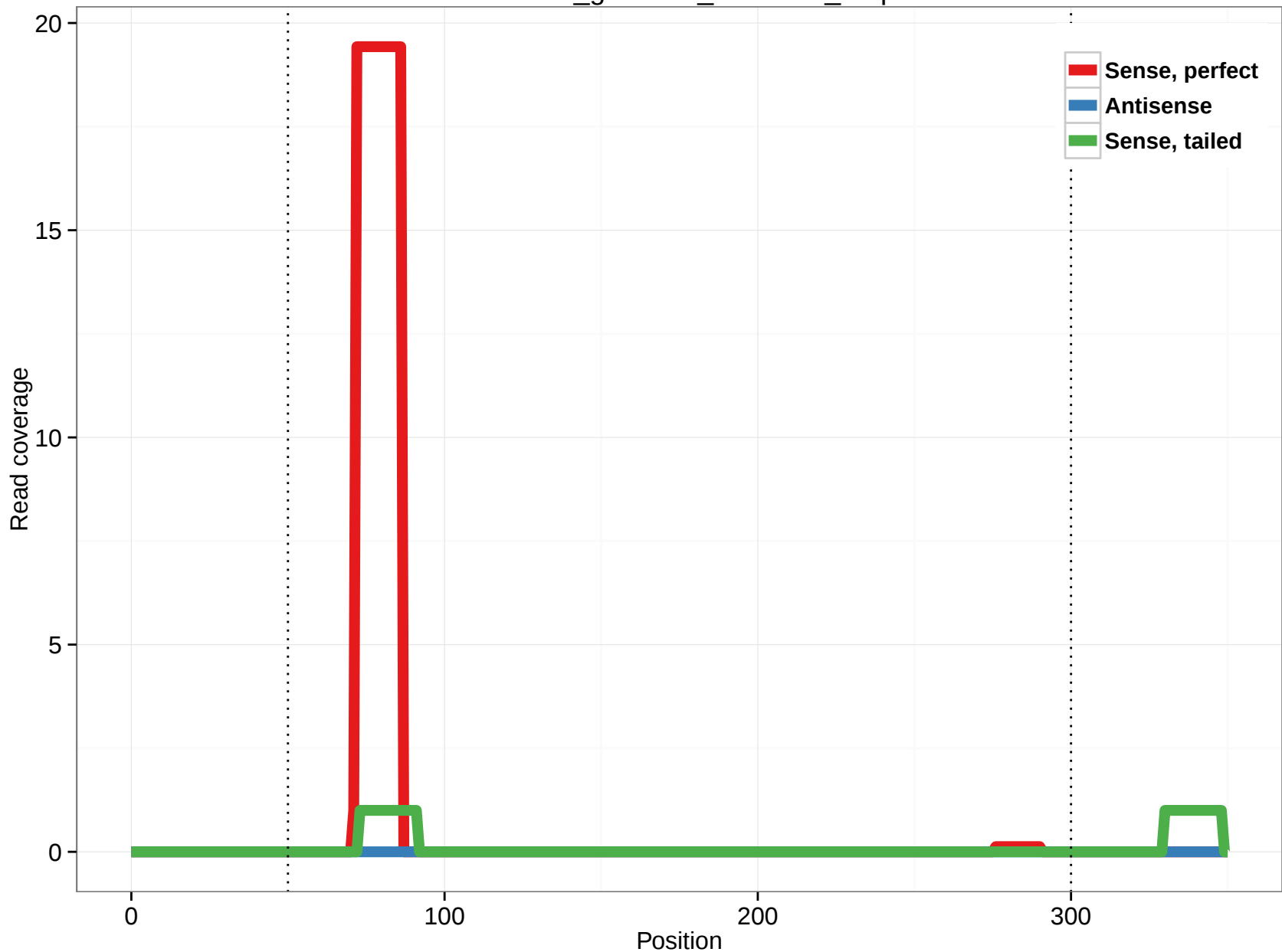
rheMac3_genscan_chr11.24_1.3p
