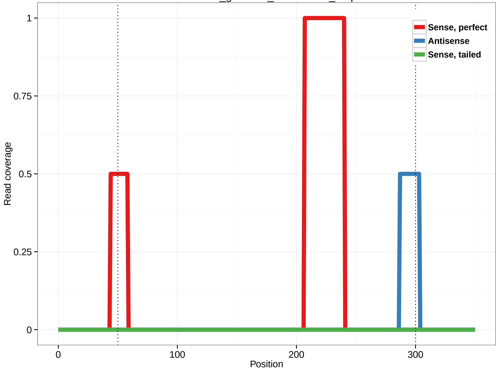
rheMac3_genscan_chr11.2497_3.3p
