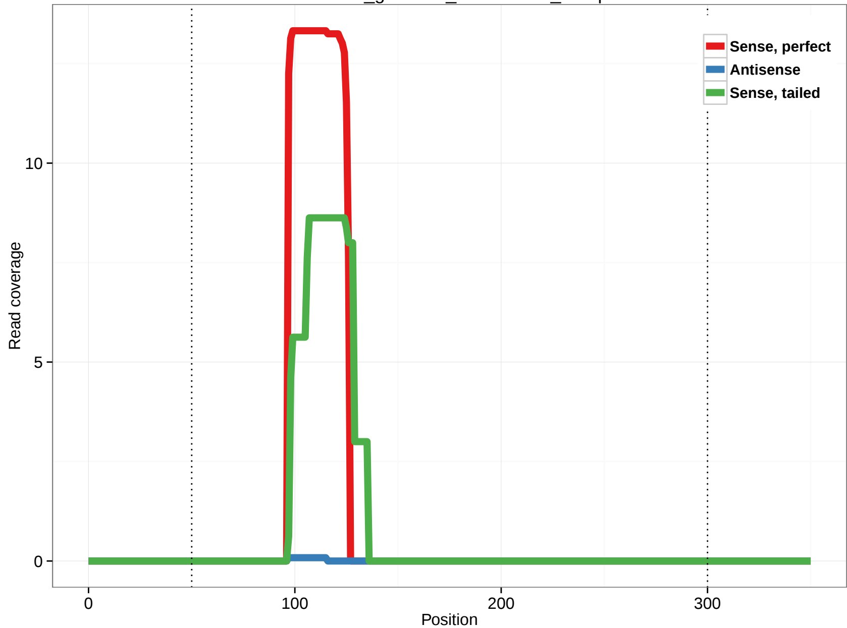
rheMac3_genscan_chr11.2462_18.5p
