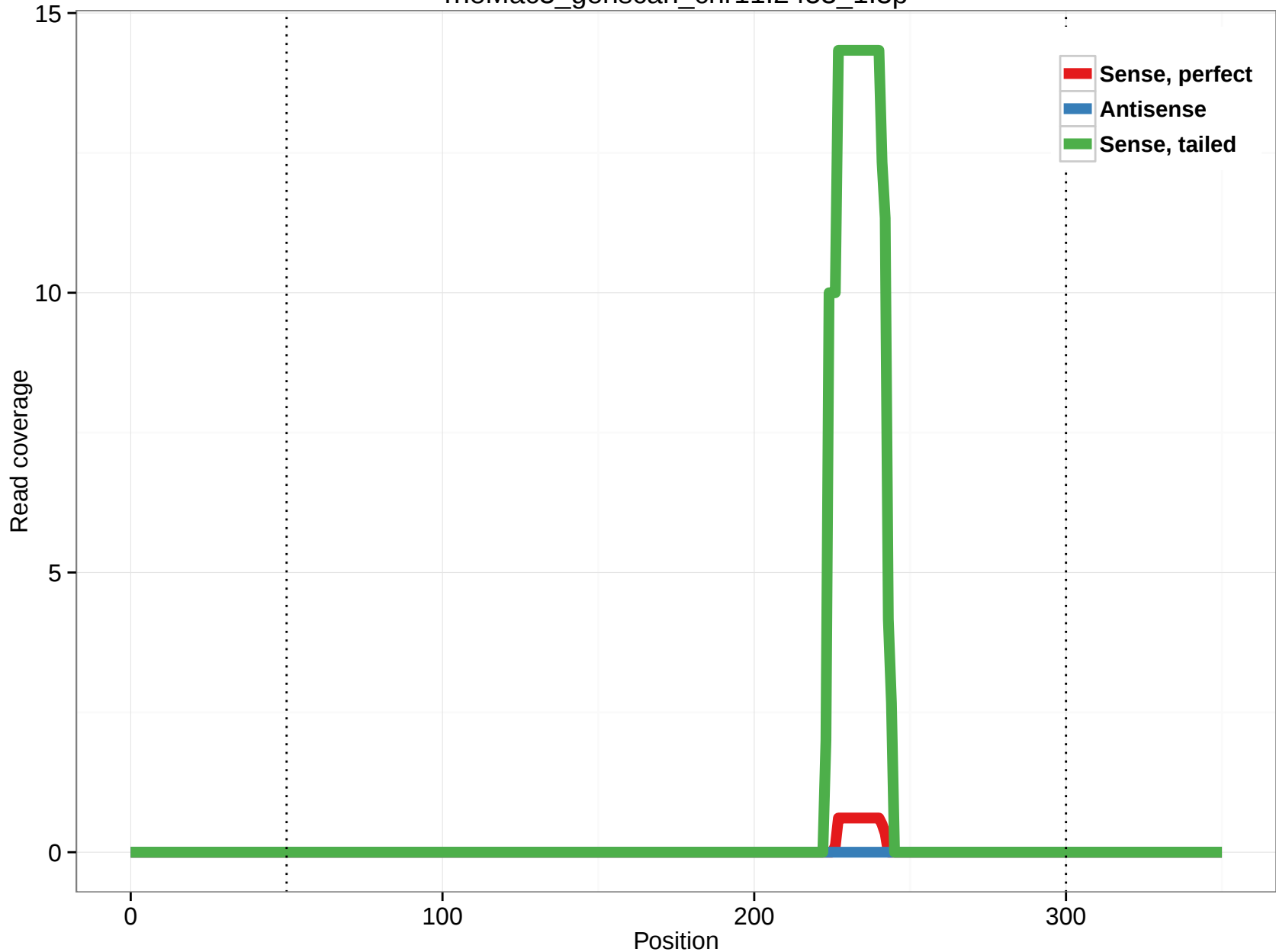
rheMac3_genscan_chr11.2453_1.3p
