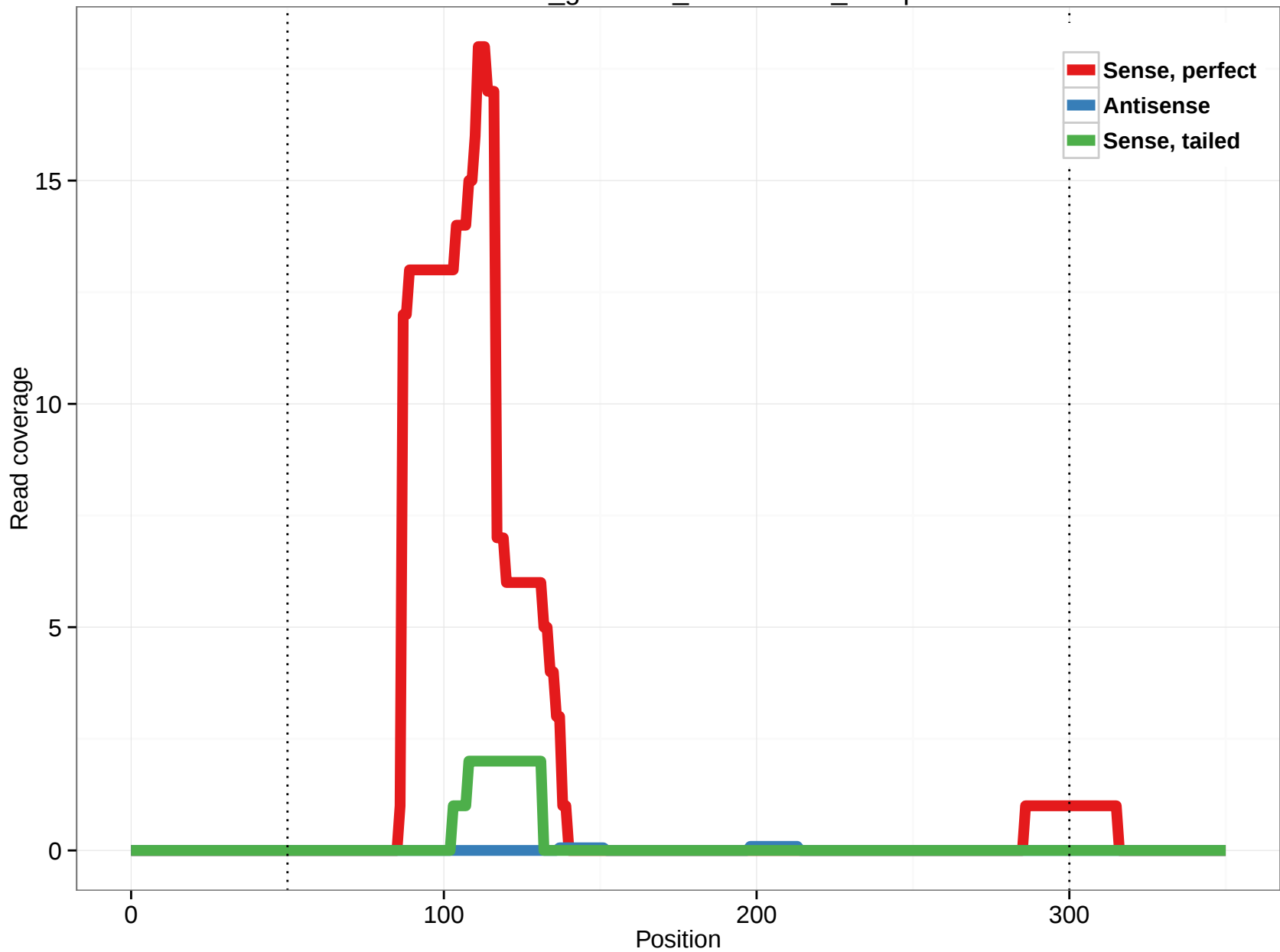
rheMac3_genscan_chr11.2437_11.5p
