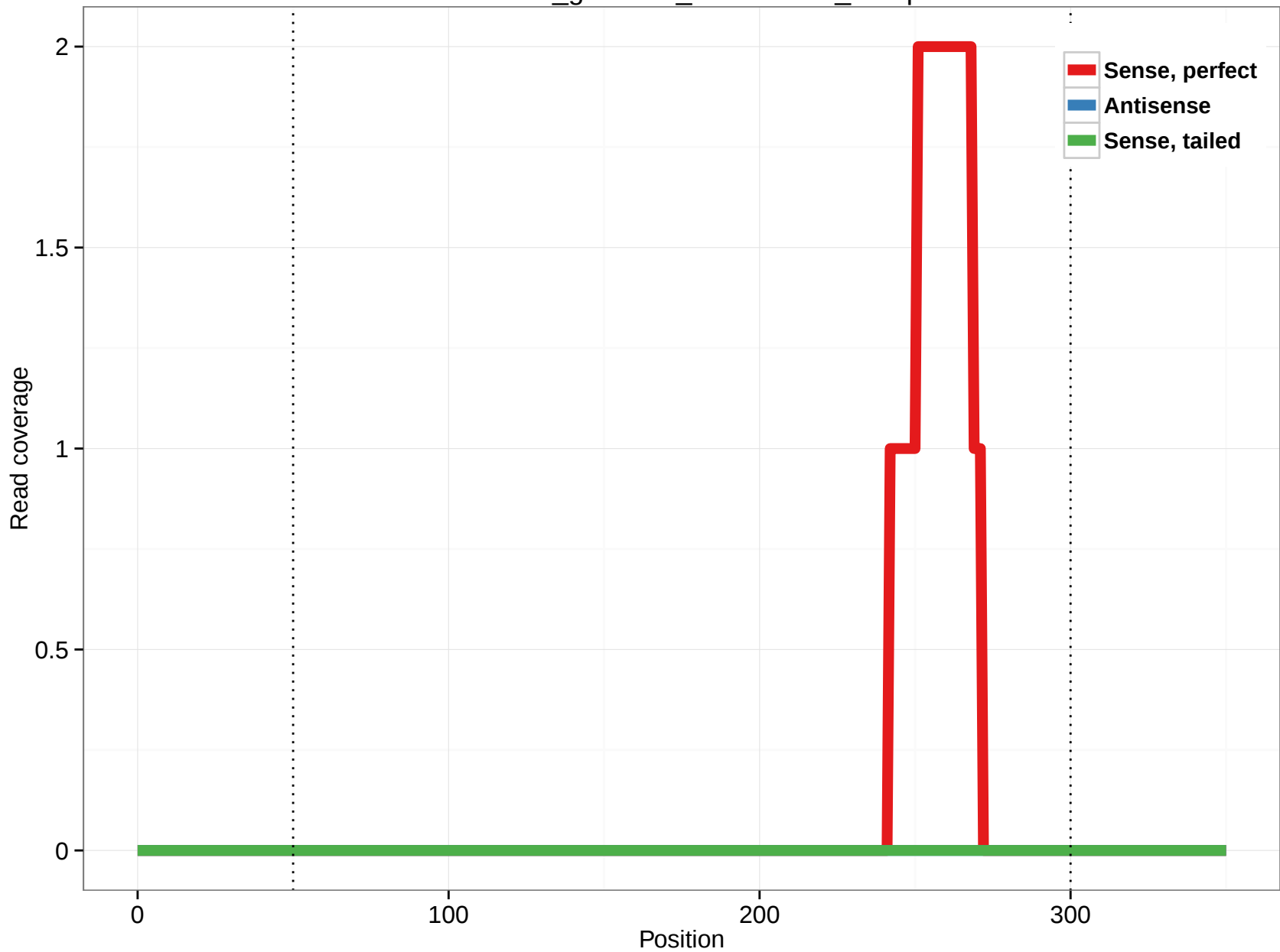
rheMac3_genscan_chr11.2351_40.3p
