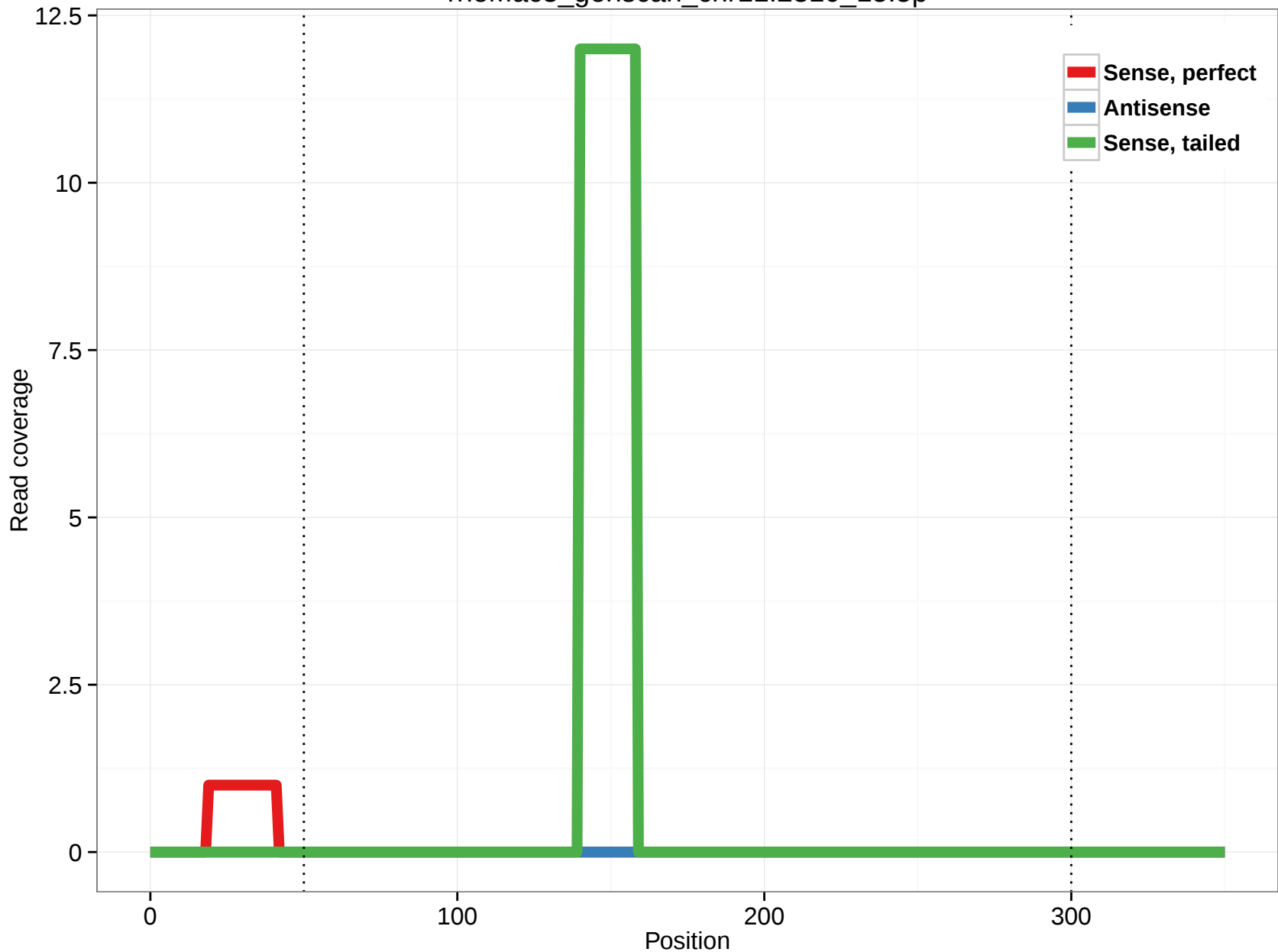
rheMac3_genscan_chr11.2310_15.5p
