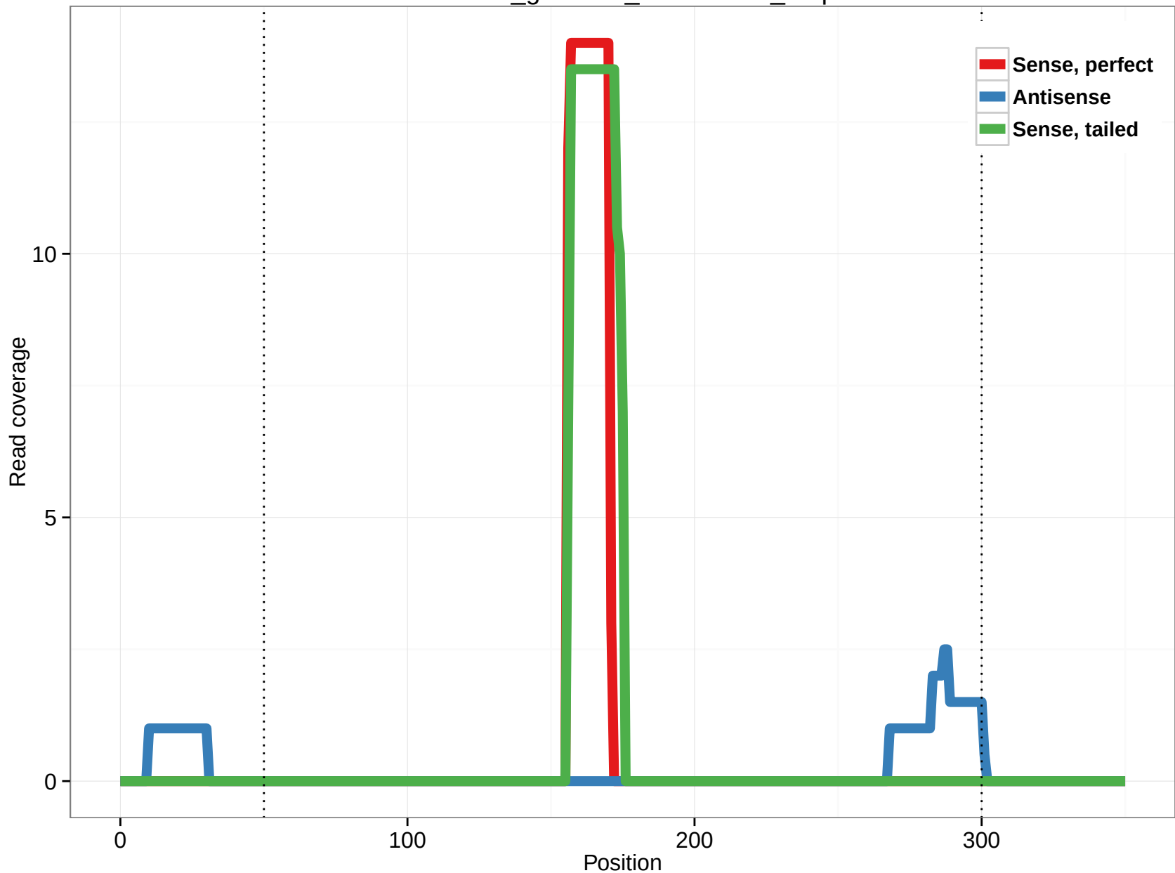
rheMac3_genscan_chr11.2291_0.5p
