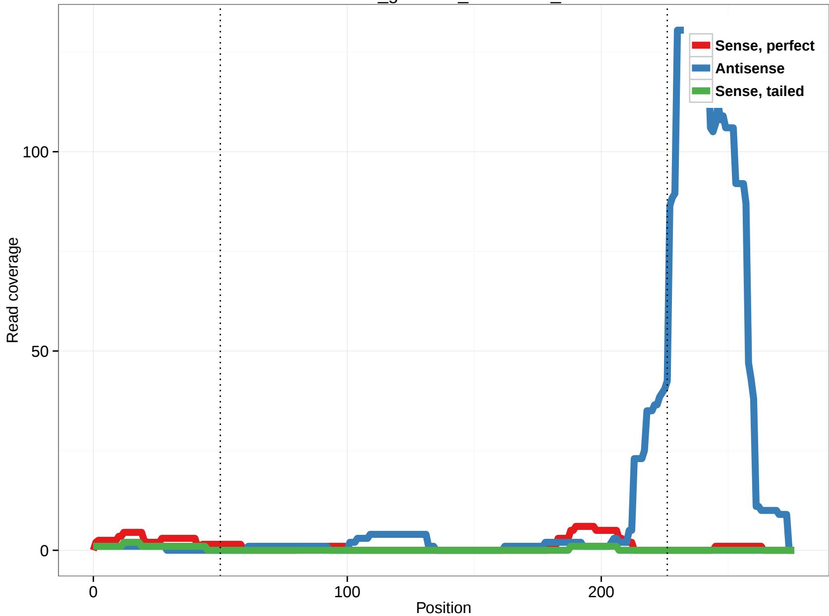
rheMac3_genscan_chr11.227_31
