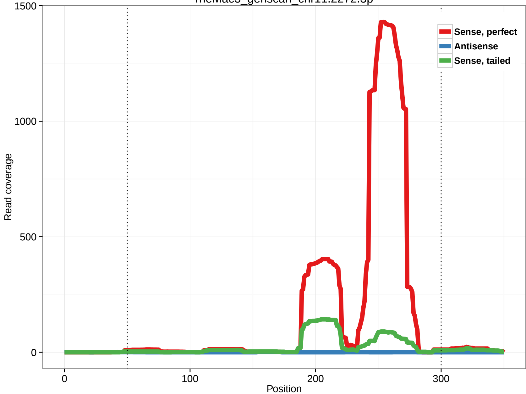
rheMac3_genscan_chr11.2272.3p
