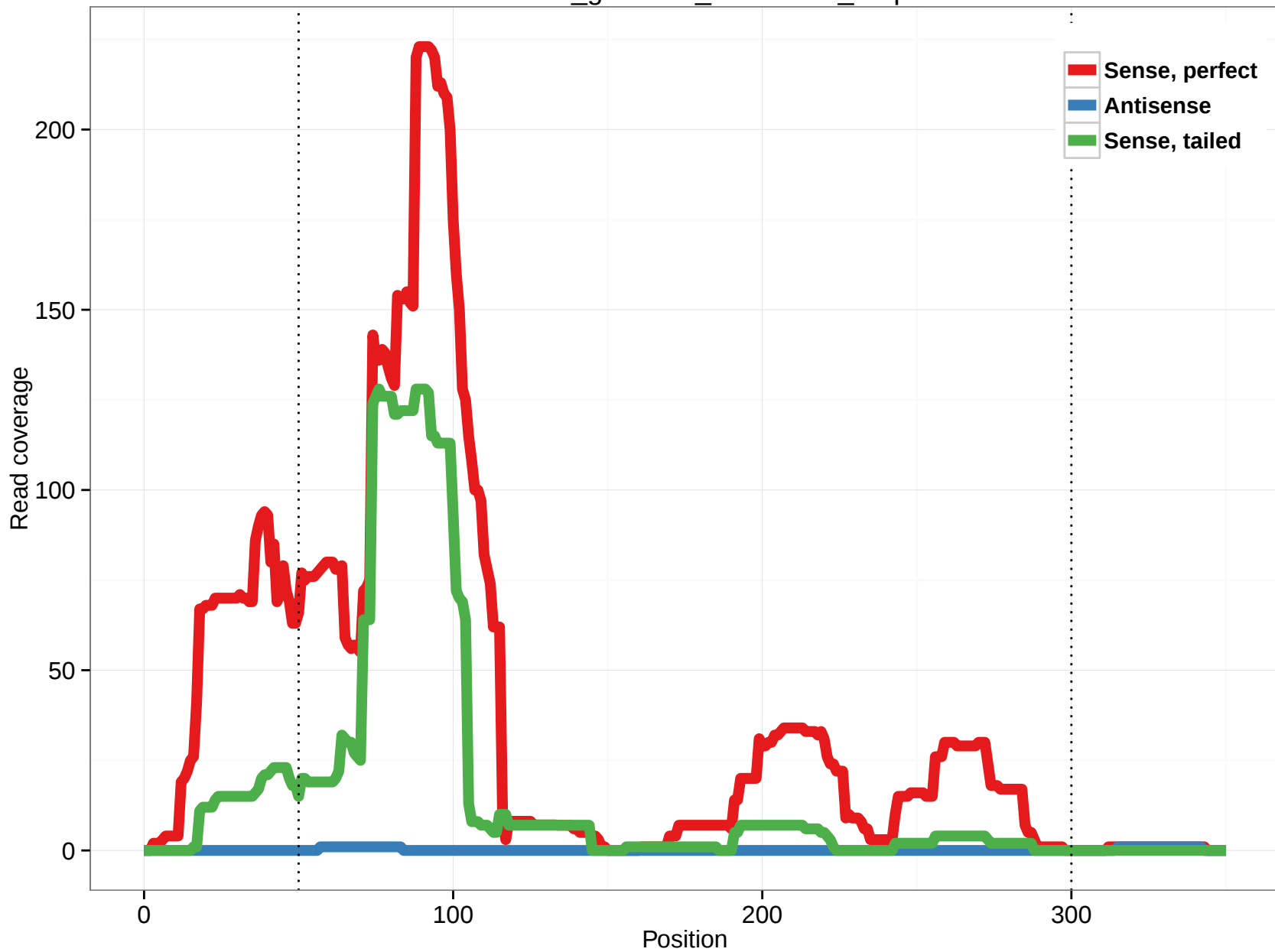
rheMac3_genscan_chr11.225_7.5p
