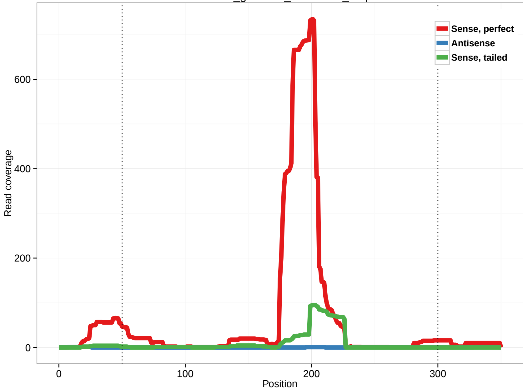
rheMac3_genscan_chr11.225_5.3p
