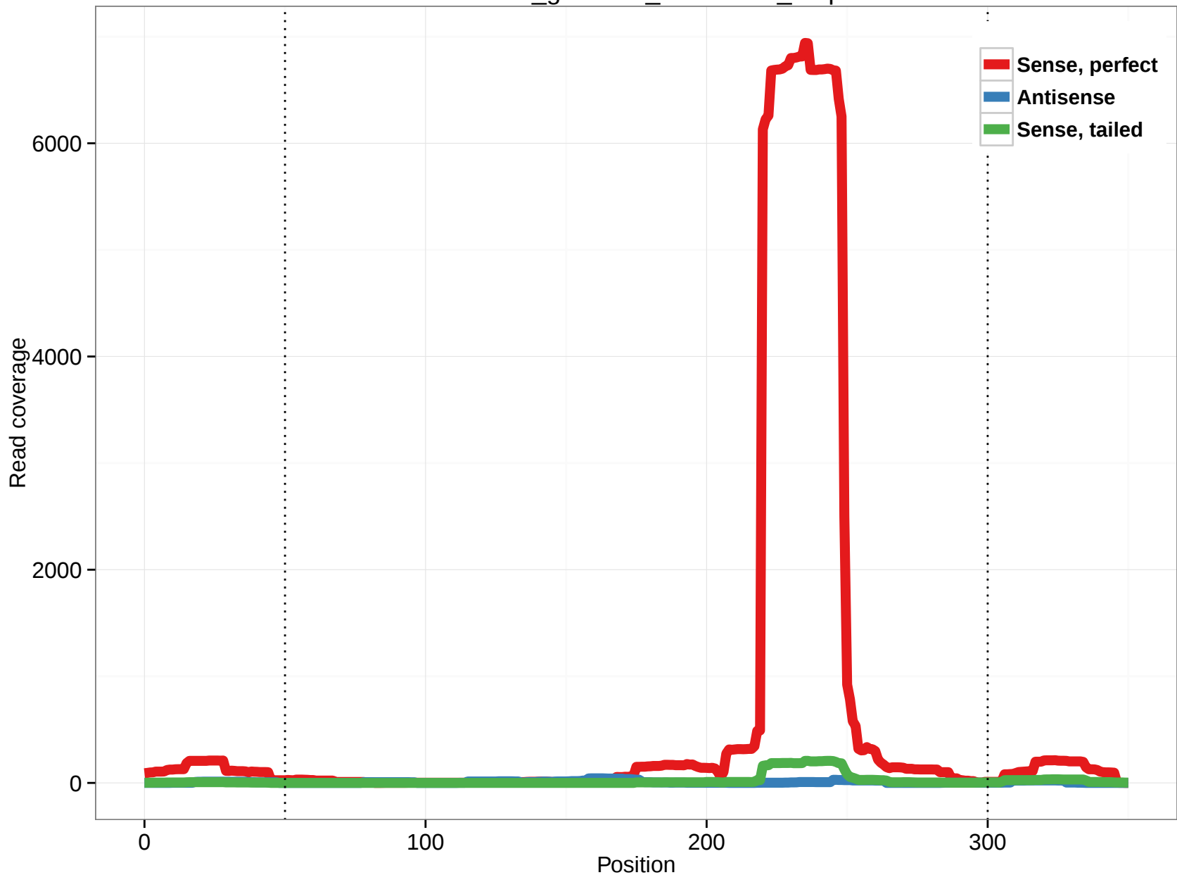
rheMac3_genscan_chr11.225_4.5p
