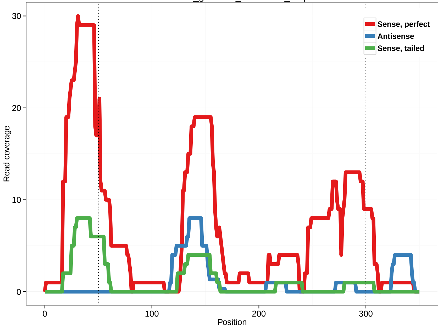
rheMac3_genscan_chr11.225_3.5p
