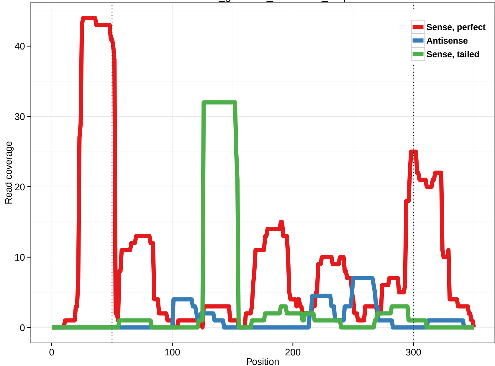
rheMac3_genscan_chr11.225_2.3p
