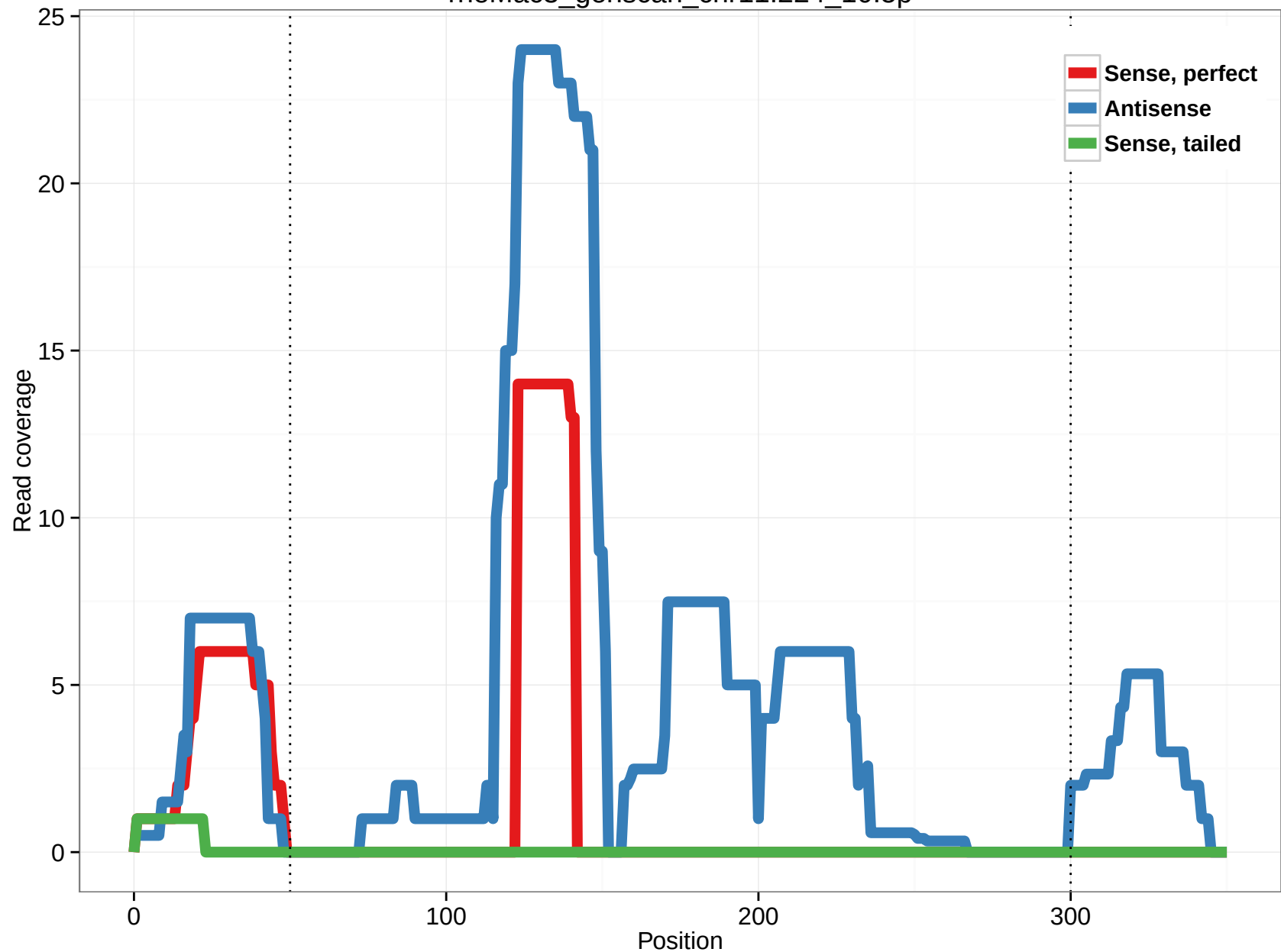
rheMac3_genscan_chr11.224_10.5p
