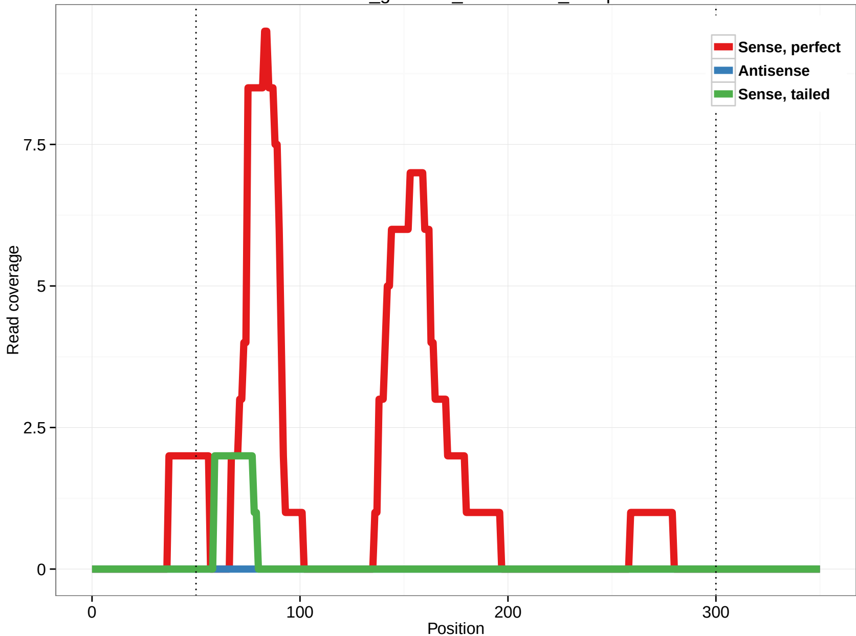
rheMac3_genscan_chr11.2235_20.3p
