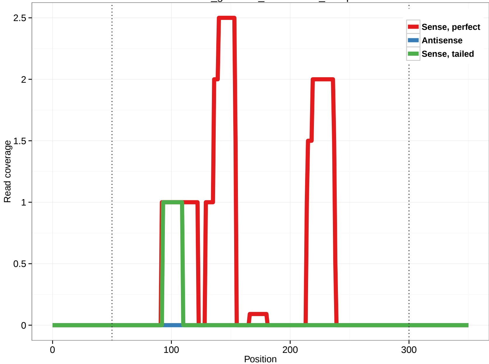
rheMac3_genscan_chr11.2212_14.5p
