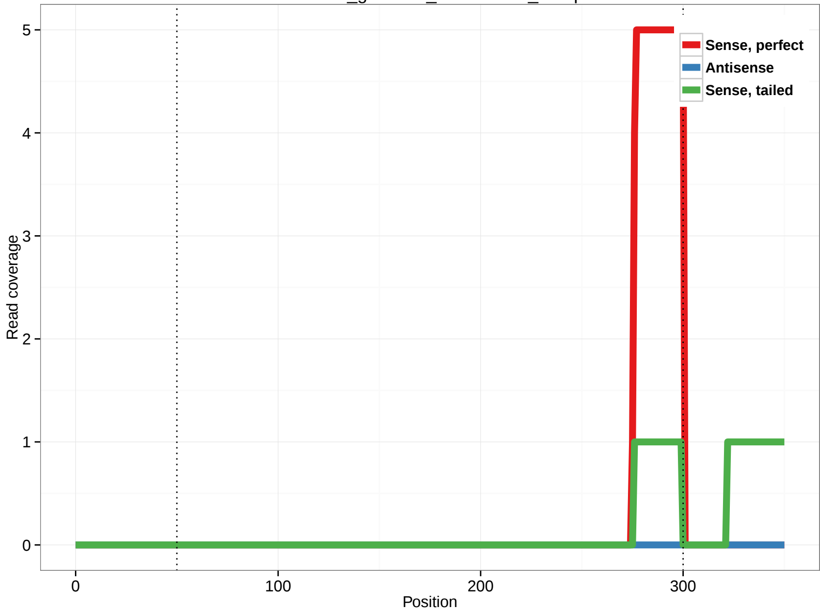
rheMac3_genscan_chr11.2204_30.3p
