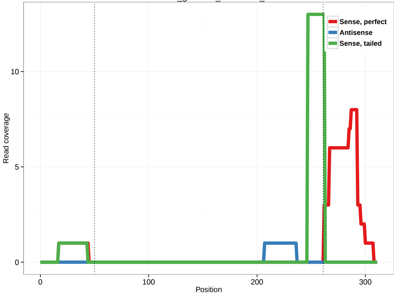
rheMac3_genscan_chr11.215_45
