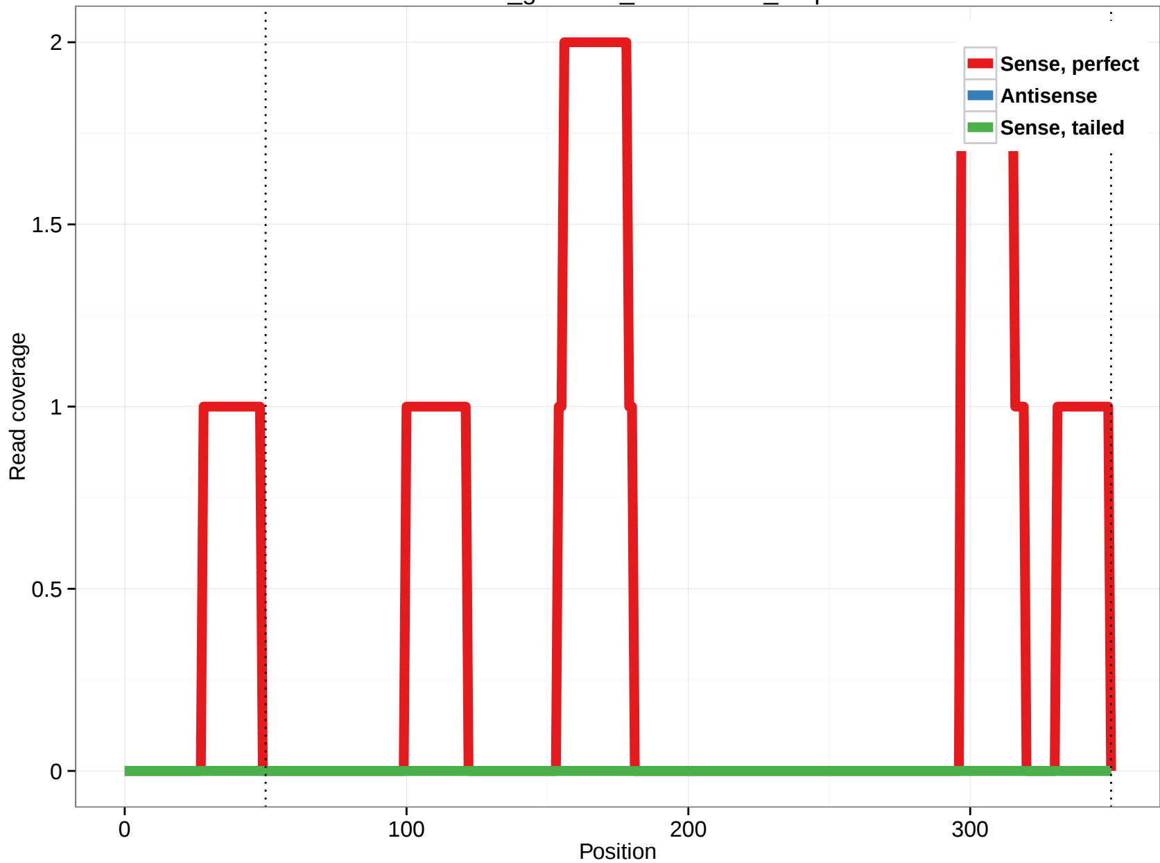
rheMac3_genscan_chr11.2158_2.5p
