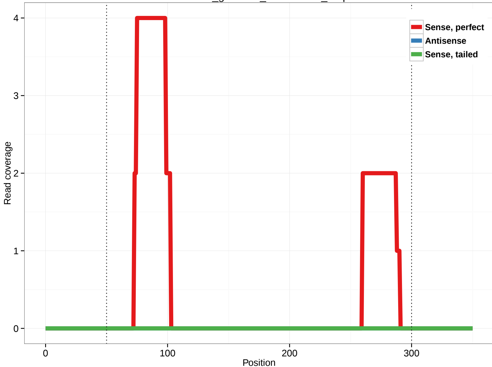
rheMac3_genscan_chr11.2158_1.5p
