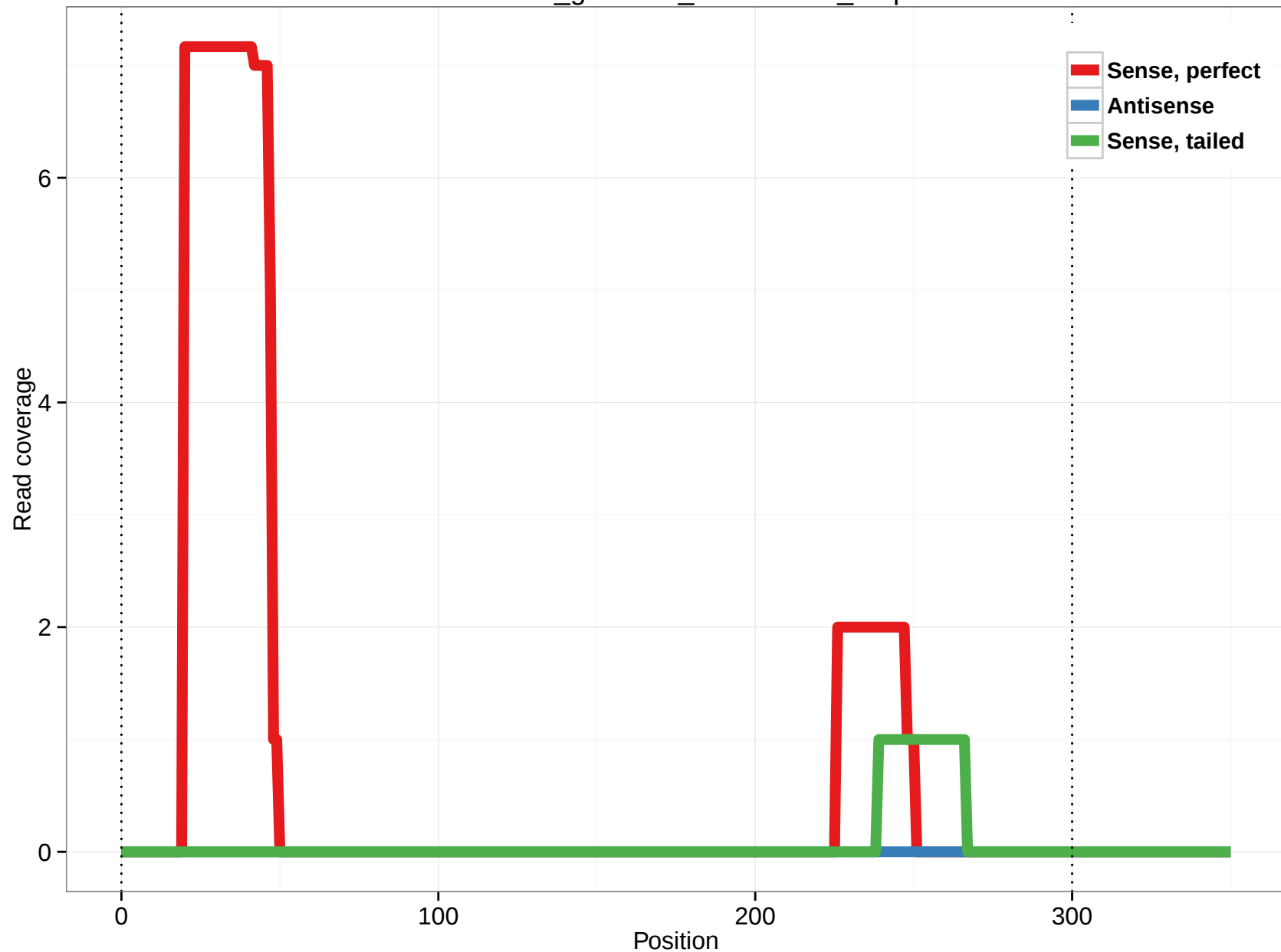
rheMac3_genscan_chr11.2158_0.3p
