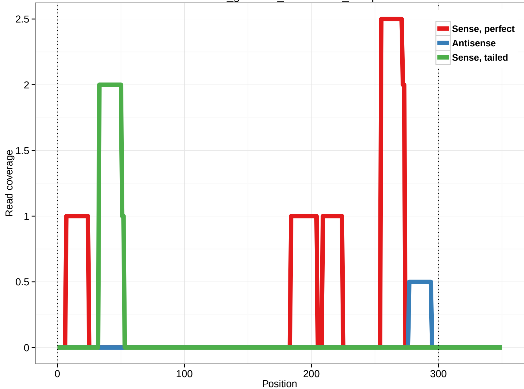
rheMac3_genscan_chr11.2132_23.3p
