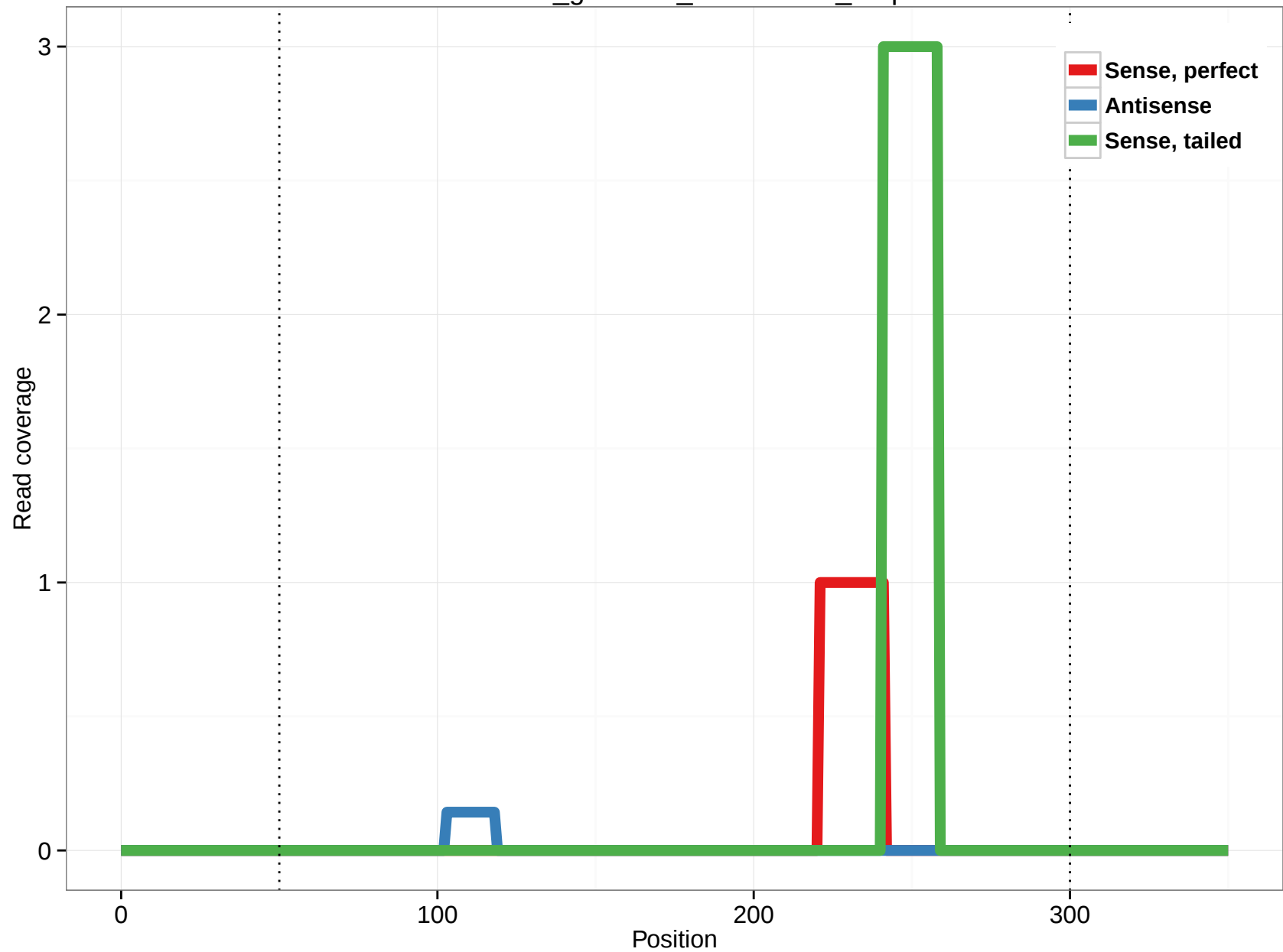
rheMac3_genscan_chr11.2100_4.3p
