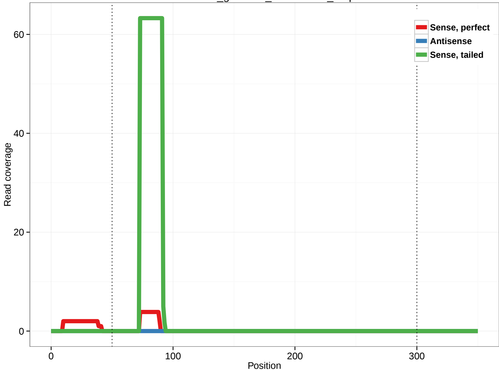
rheMac3_genscan_chr11.2073_4.5p
