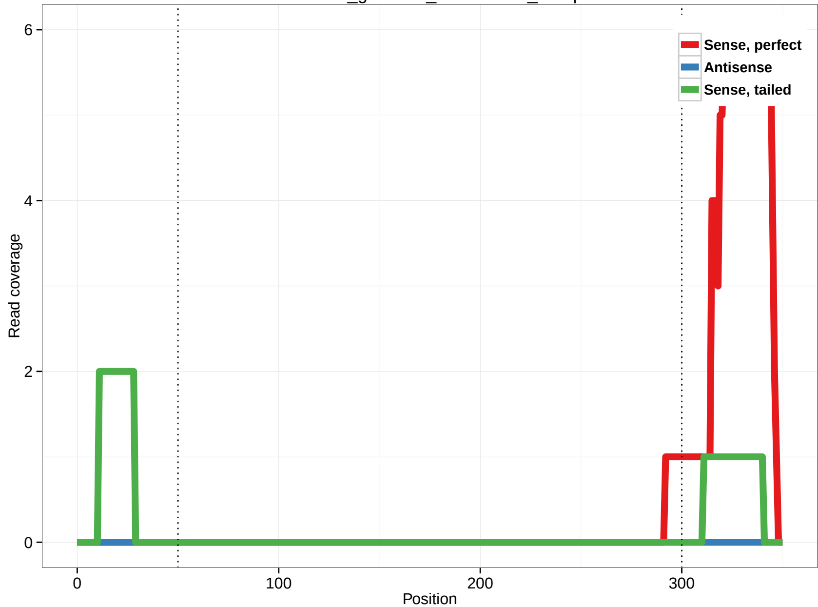
rheMac3_genscan_chr11.2073_11.3p
