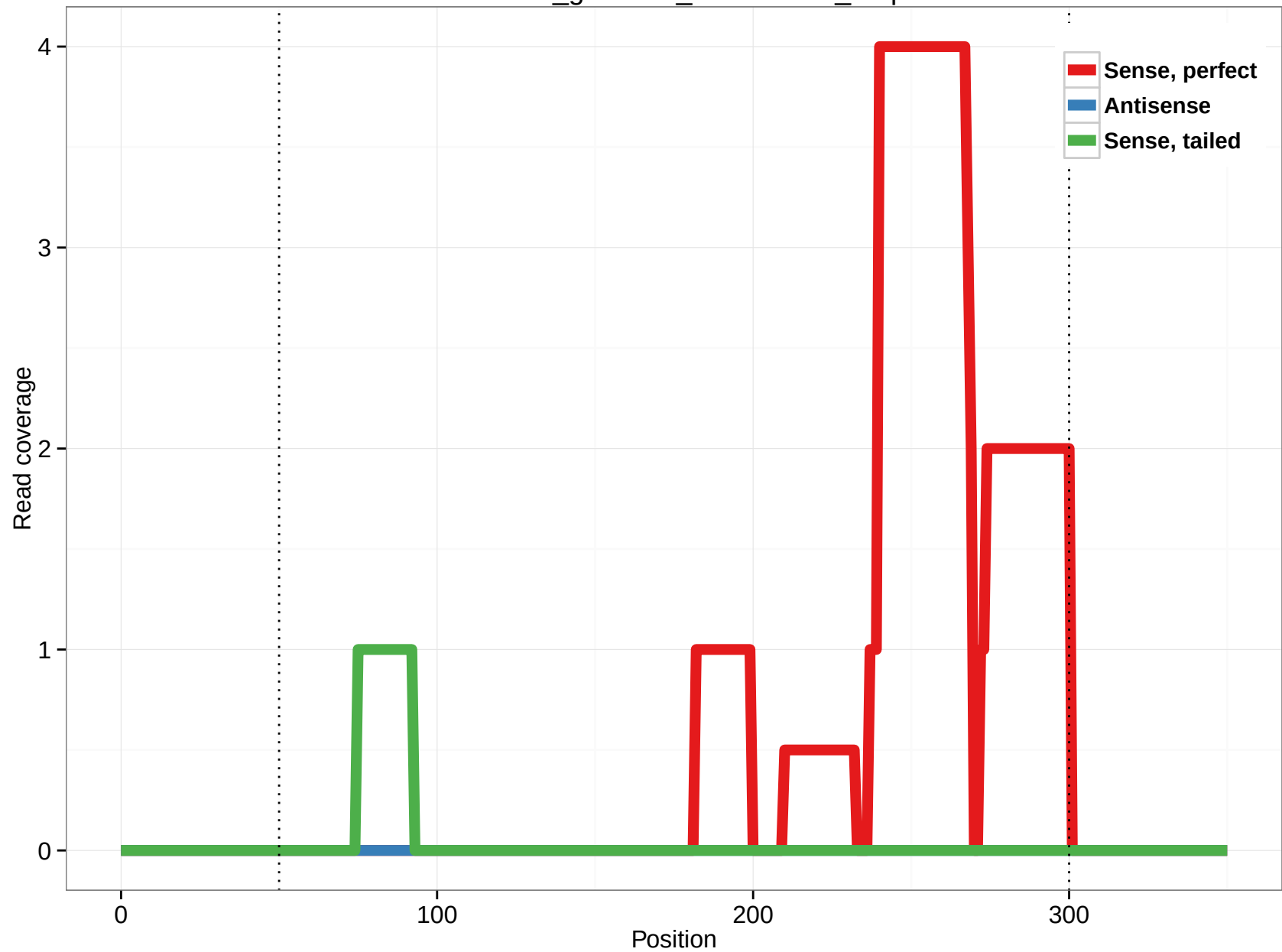
rheMac3_genscan_chr11.2072_4.3p
