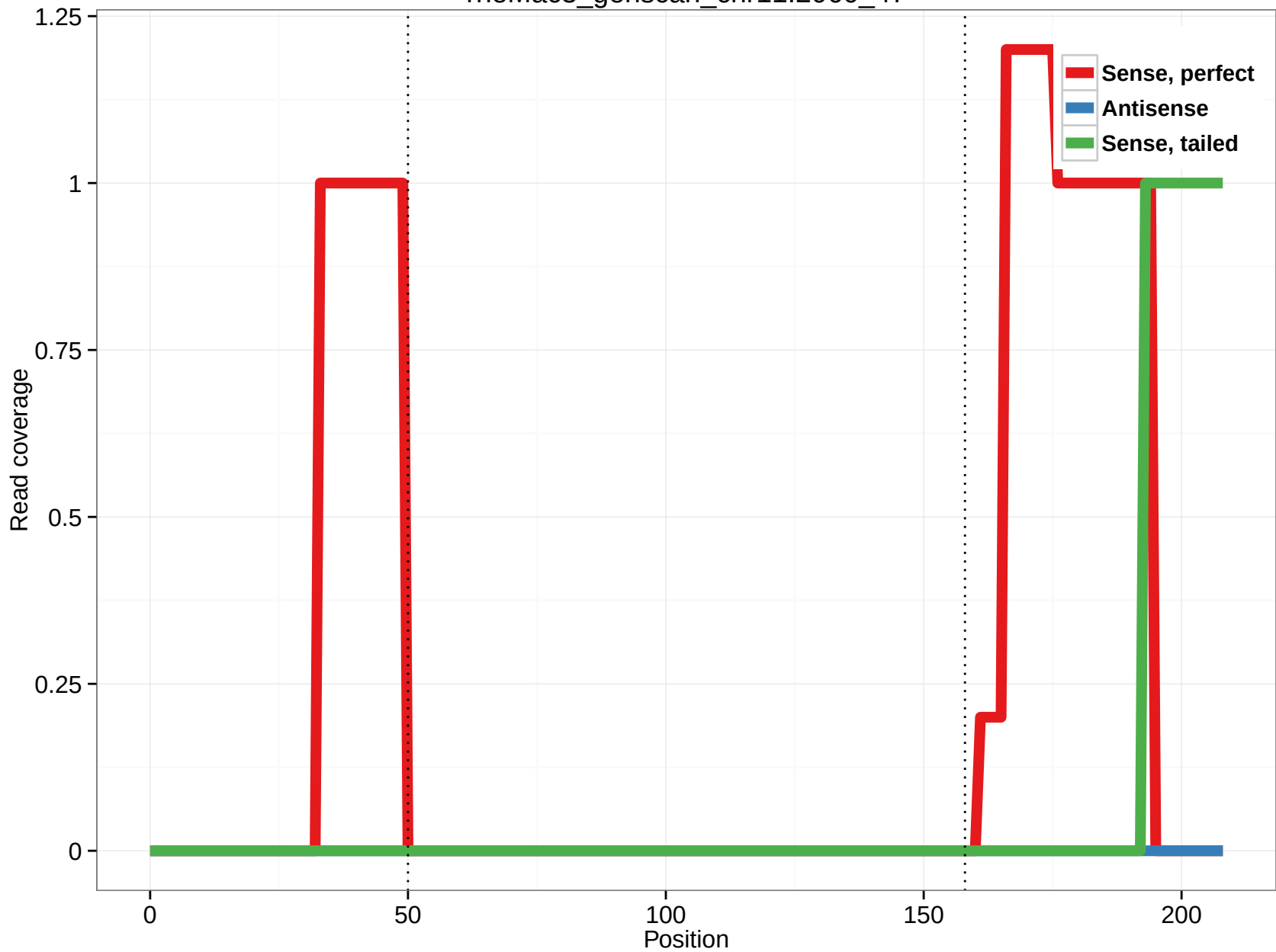
rheMac3_genscan_chr11.2060_47
