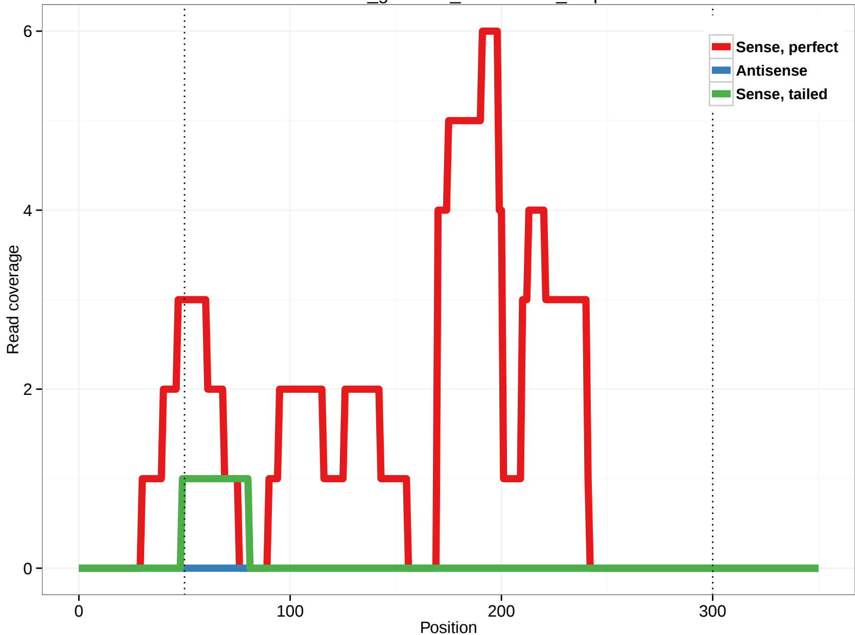
rheMac3_genscan_chr11.2038_3.5p
