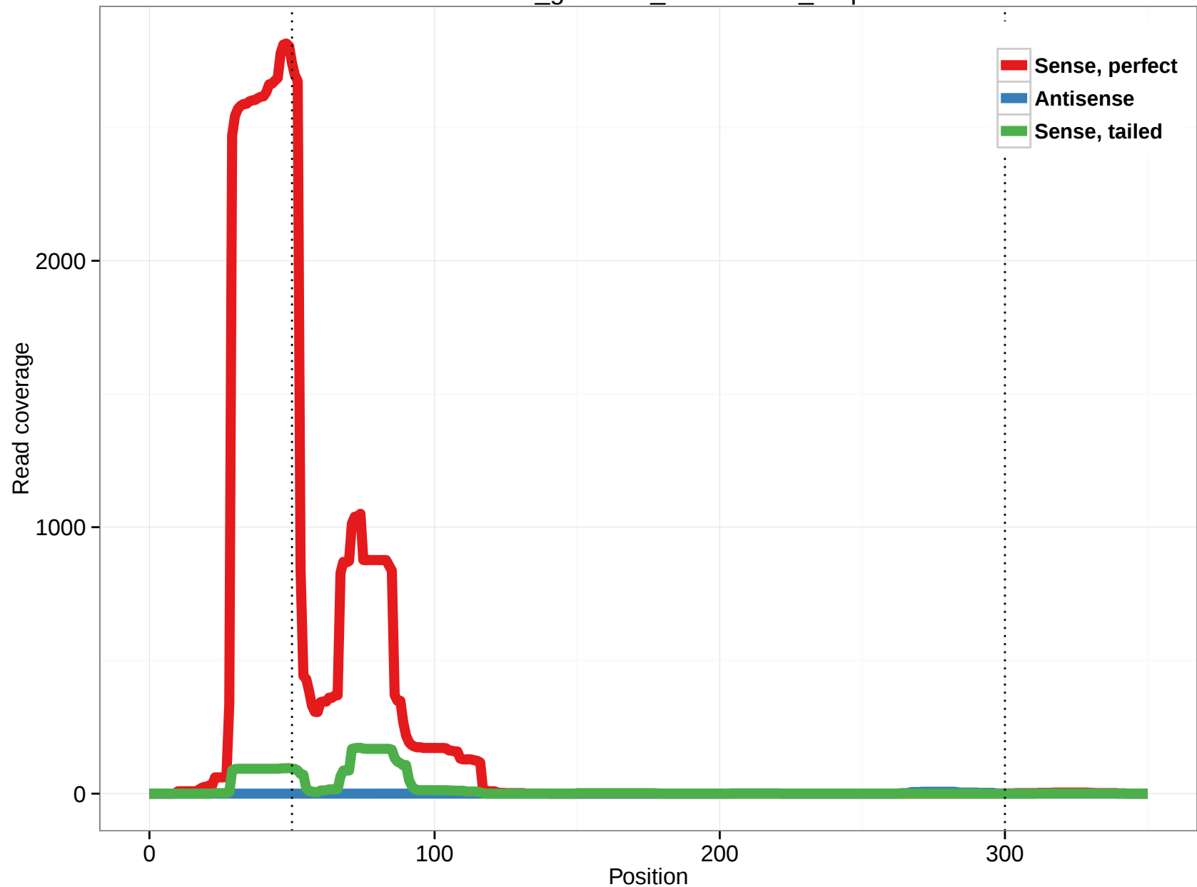
rheMac3_genscan_chr11.1877_6.3p
