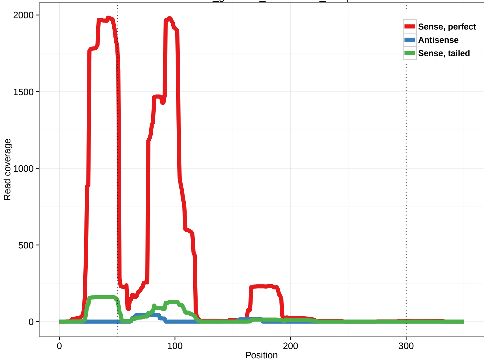
rheMac3_genscan_chr11.1877_16.5p
