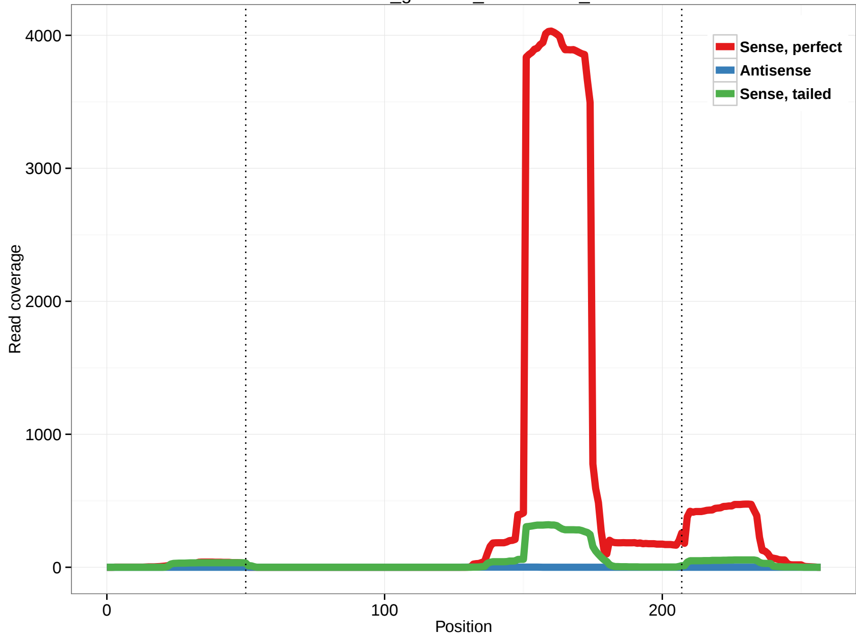
rheMac3_genscan_chr11.1877_14
