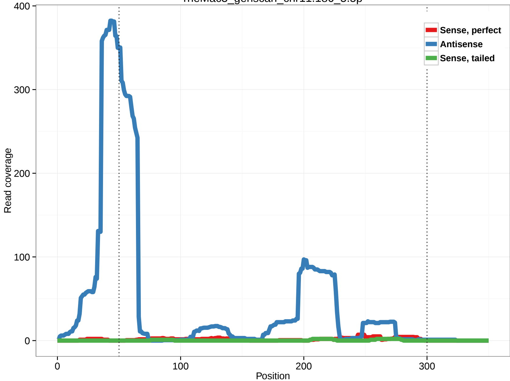
rheMac3_genscan_chr11.186_5.5p
