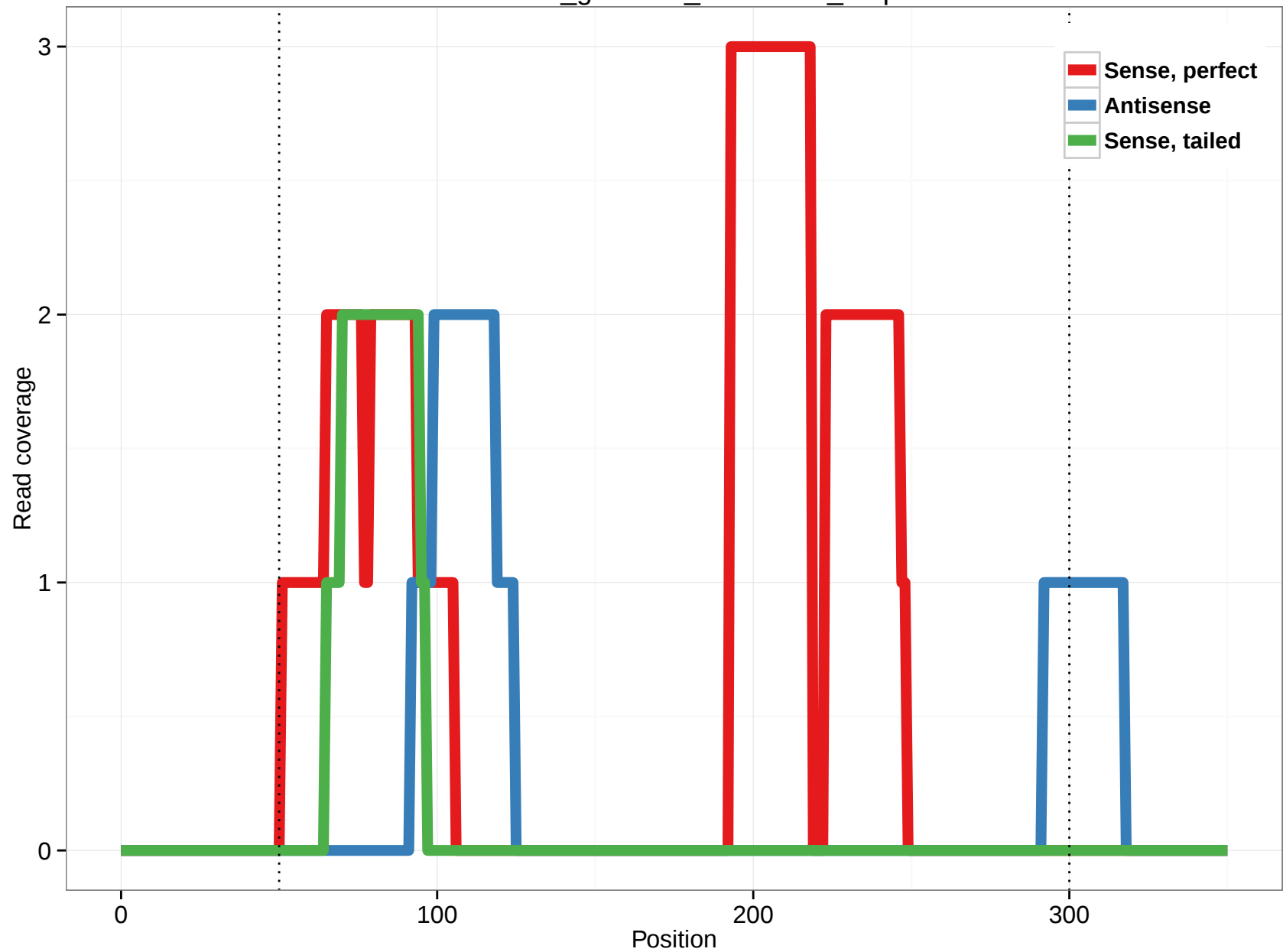
rheMac3_genscan_chr11.186_5.3p
