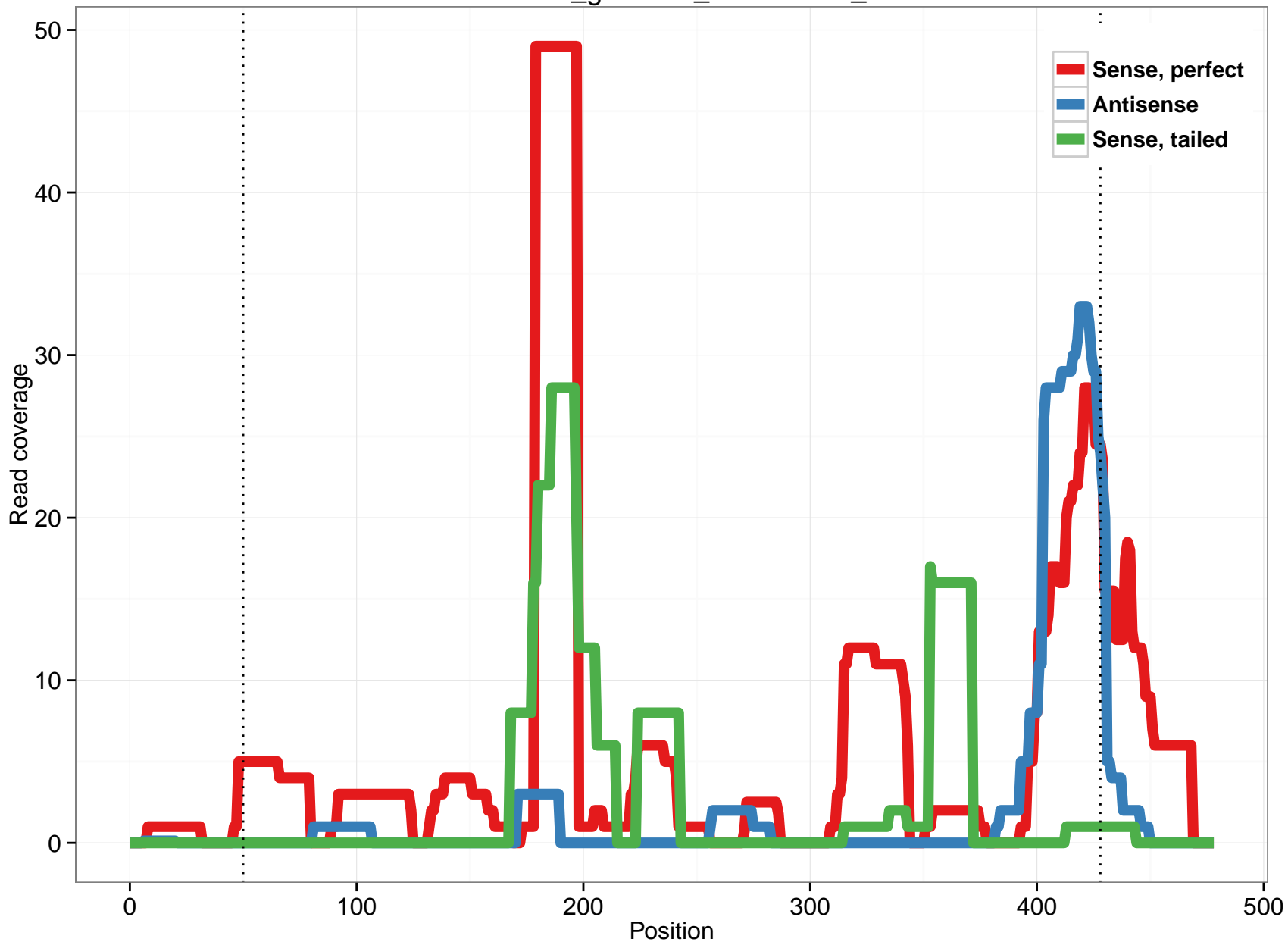
rheMac3_genscan_chr11.1855_1
