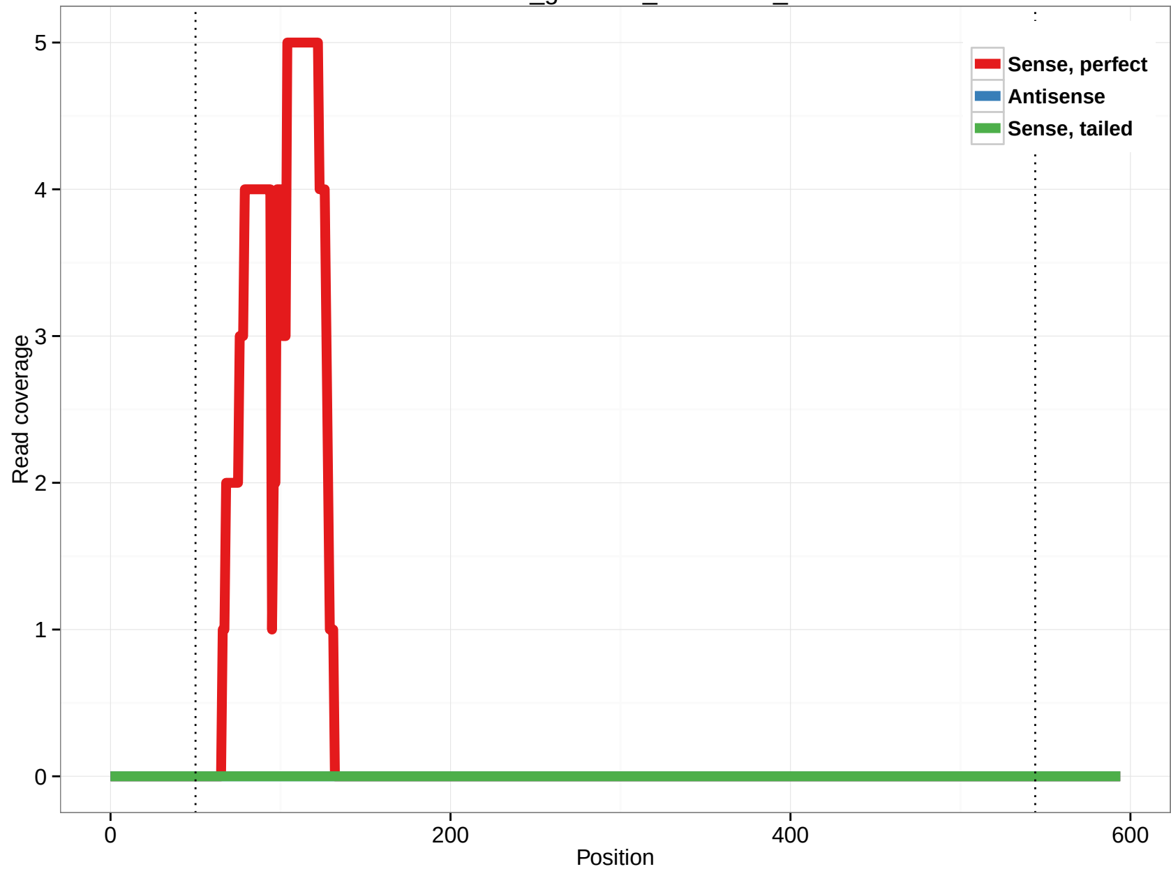
rheMac3_genscan_chr11.184_5
