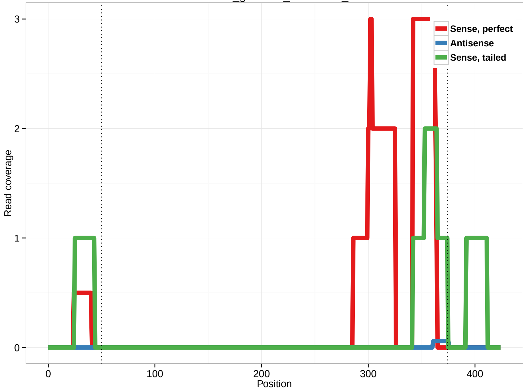
rheMac3_genscan_chr11.180_12
