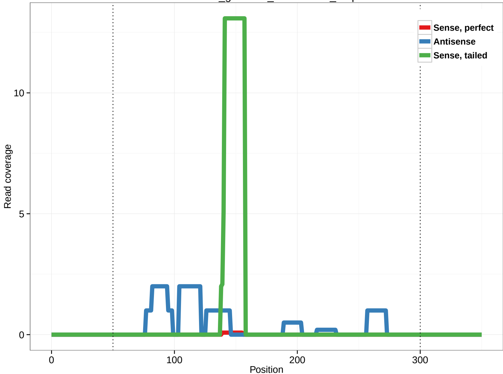
rheMac3_genscan_chr11.1807_1.5p
